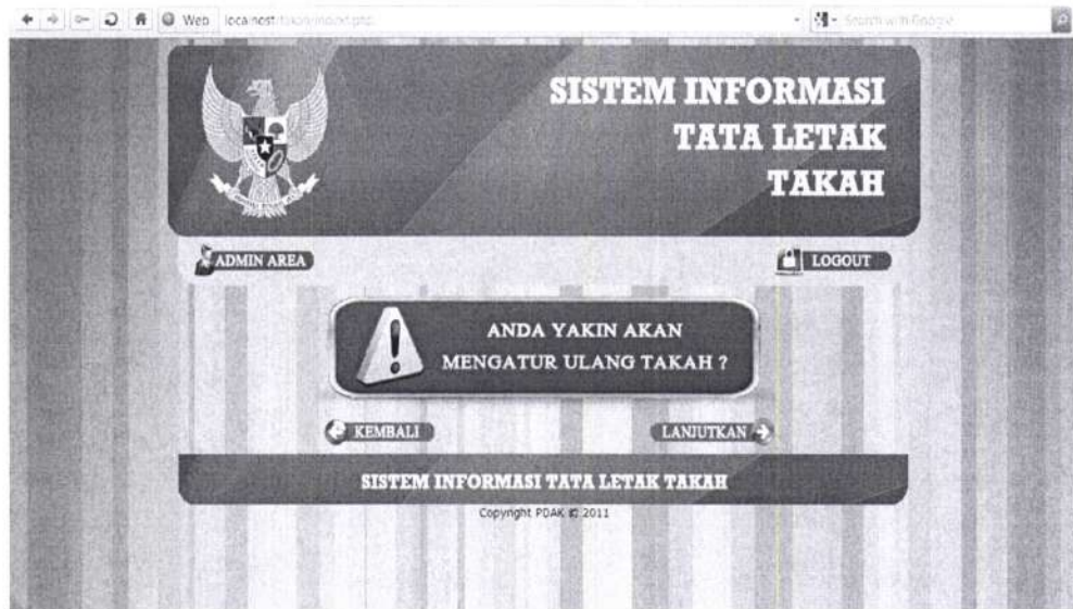
Gambar 4.2 Warning
