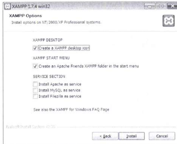
Gambar 5.3 Install XAMPP
