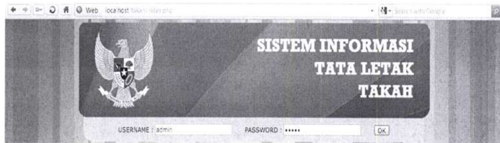
Gambar 3.1 Halaman Administrator
