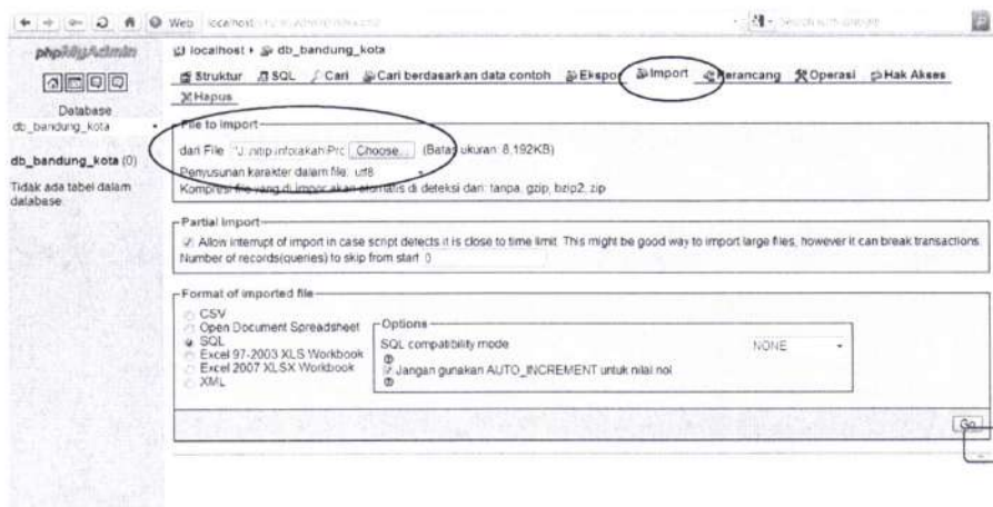
Gambar 5.9 Impor Data
