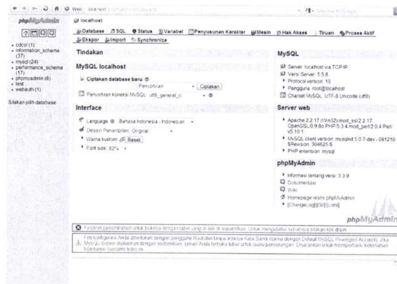
Gambar 5.6 Halaman phpMyAdmin
